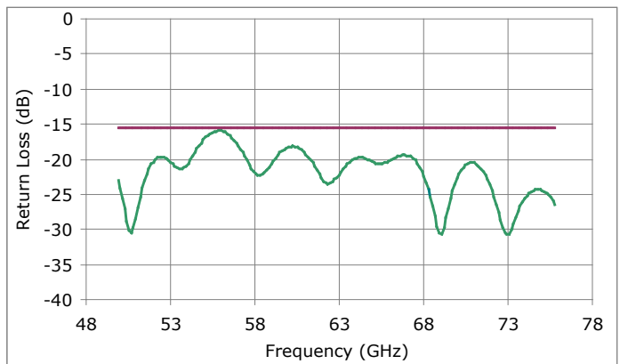
Typical Return Loss for Model 25373-WF60
