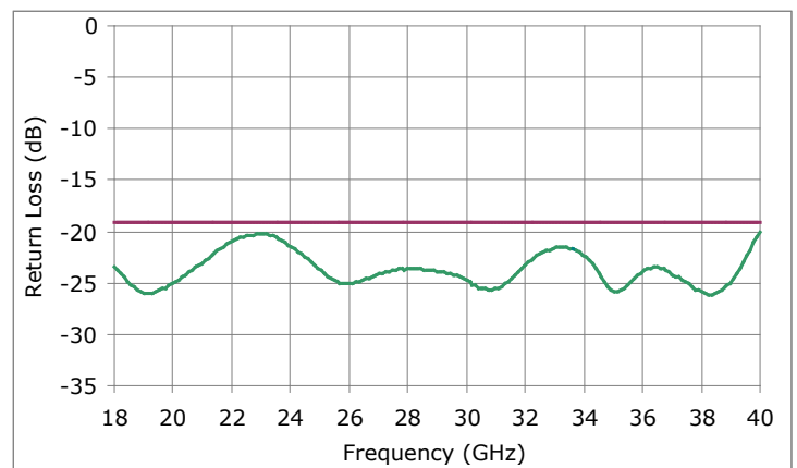
Typical Return Loss for Model WRD180093-KF20
