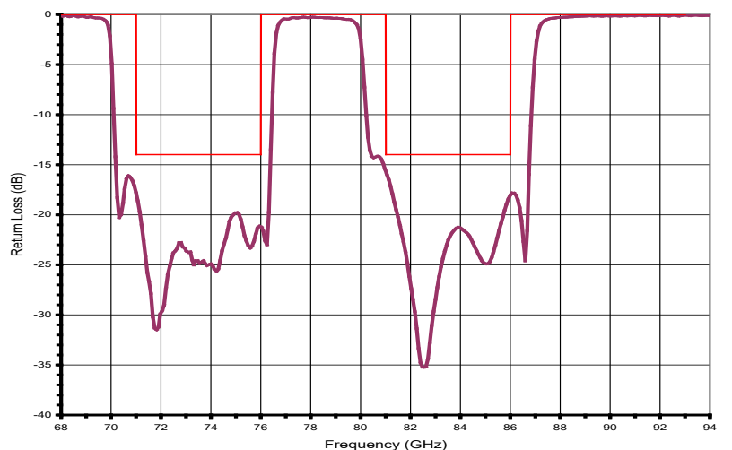
Typical Return Loss for Model 26286-AA
