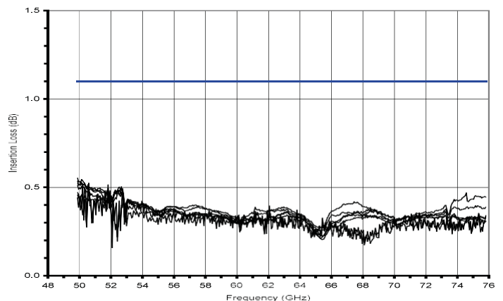
Insertion Loss for Model 25562-L300 UG-385/U
