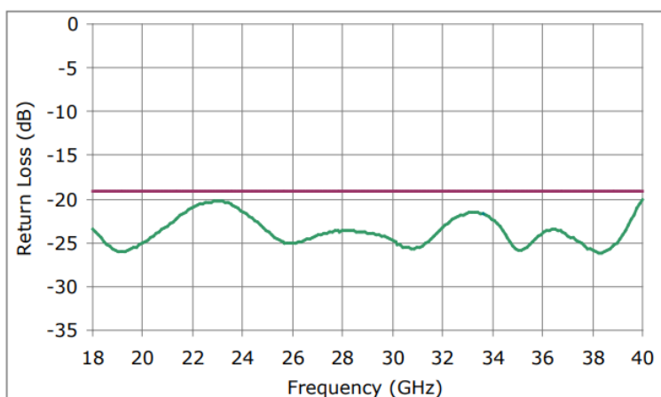
Typical Return Loss for Model WRD180093-KF20
