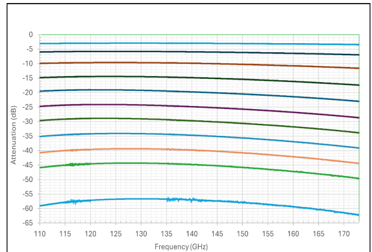
Figure: 29024 measured Attenuation vs. Frequency results
